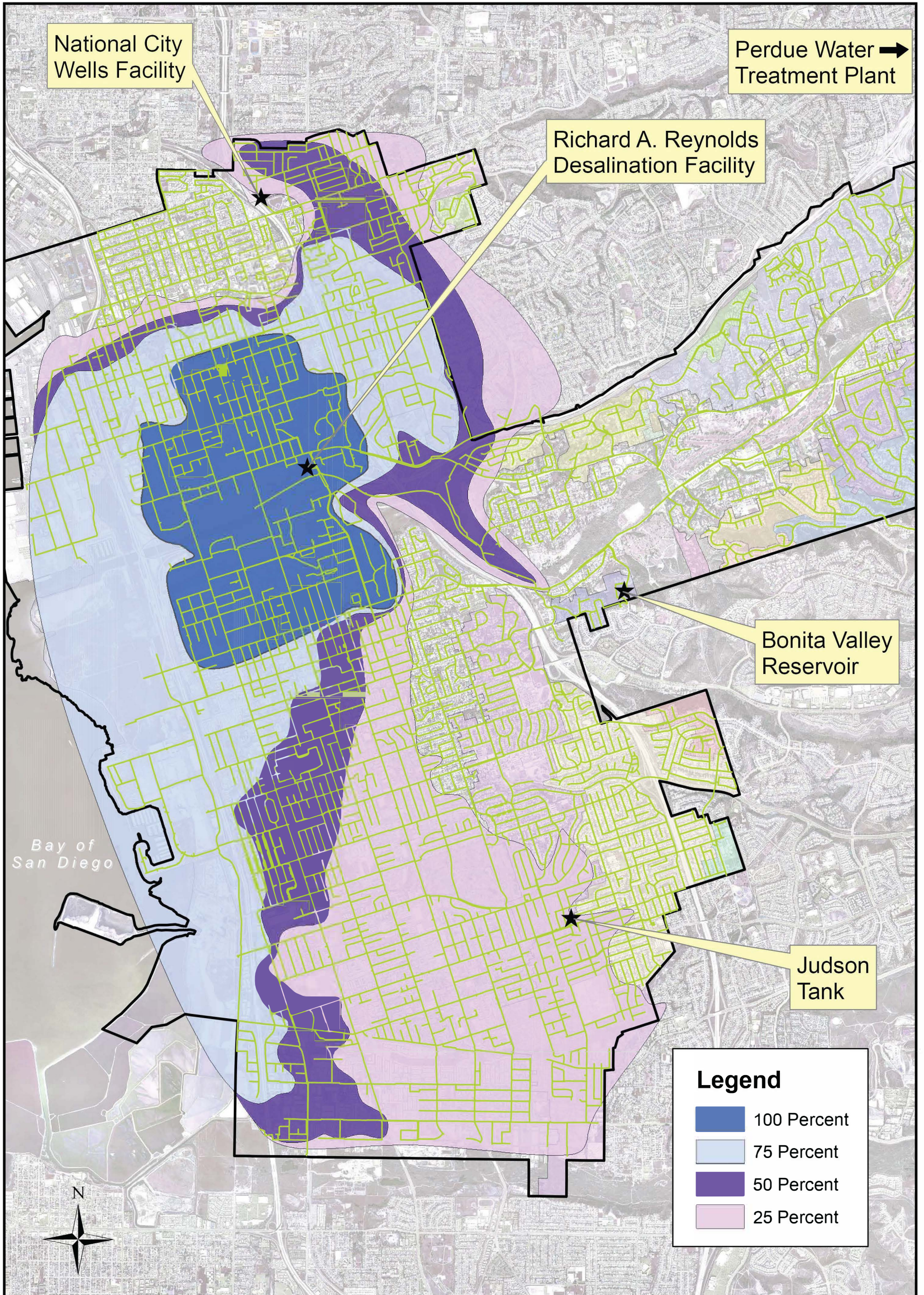
Richard A. Reynolds Desalination Water Supply Map Average percentage of water supplied from the R.A.R Desal. Facility Supply Source: Perdue 10.5 MGD, RAR Desal. 8.8 MGD, NC Wells 1.6 MGD
